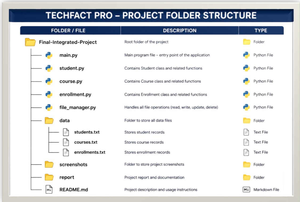
Figure 1: Project Directory Structure
