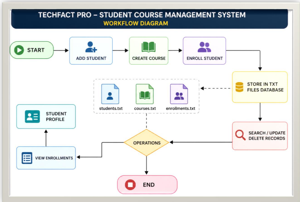
Figure 2: System Workflow Diagram
