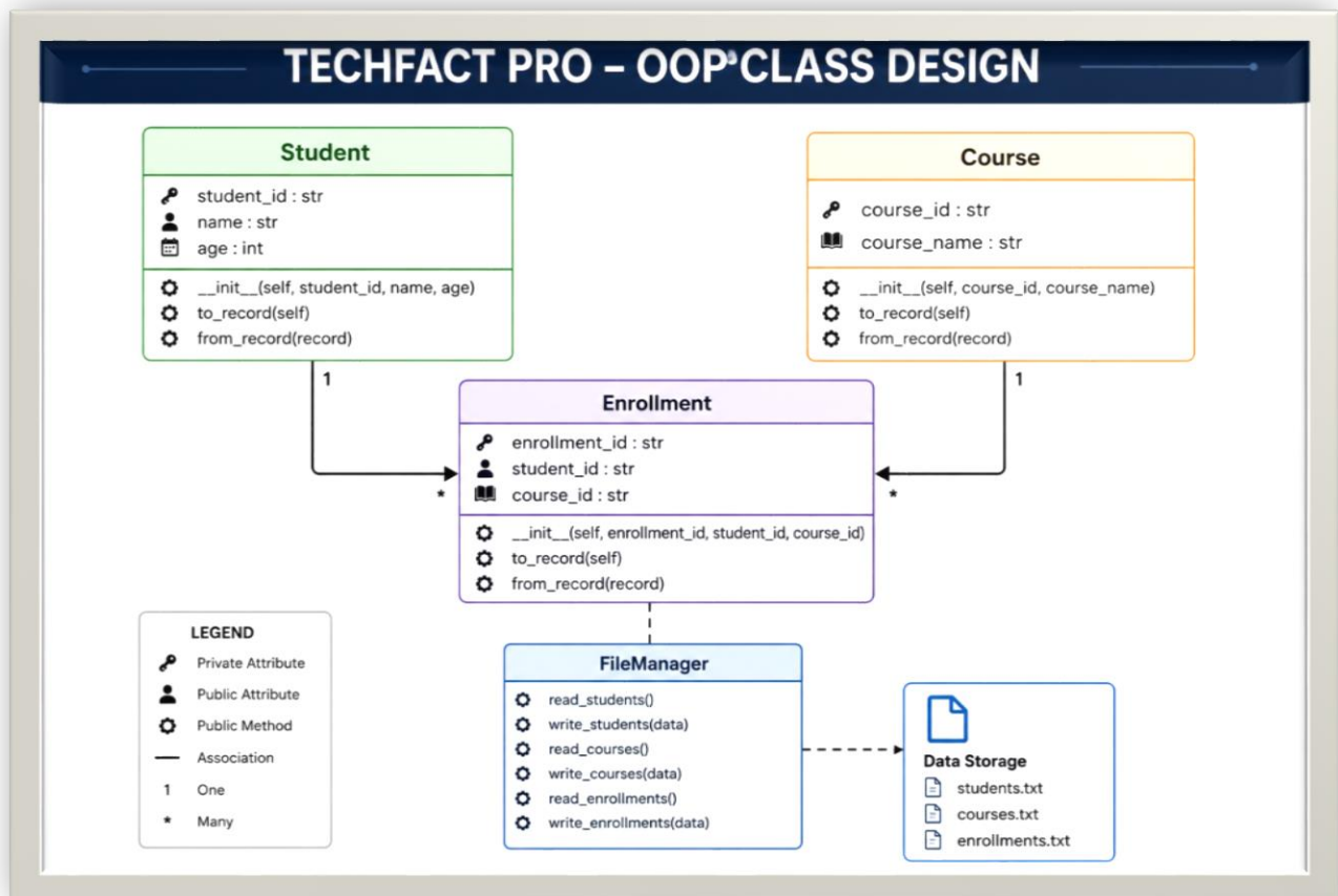
Figure 4: OOP Class Design Diagram
