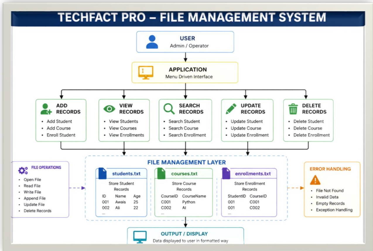
Figure 5: File Management System Architecture
